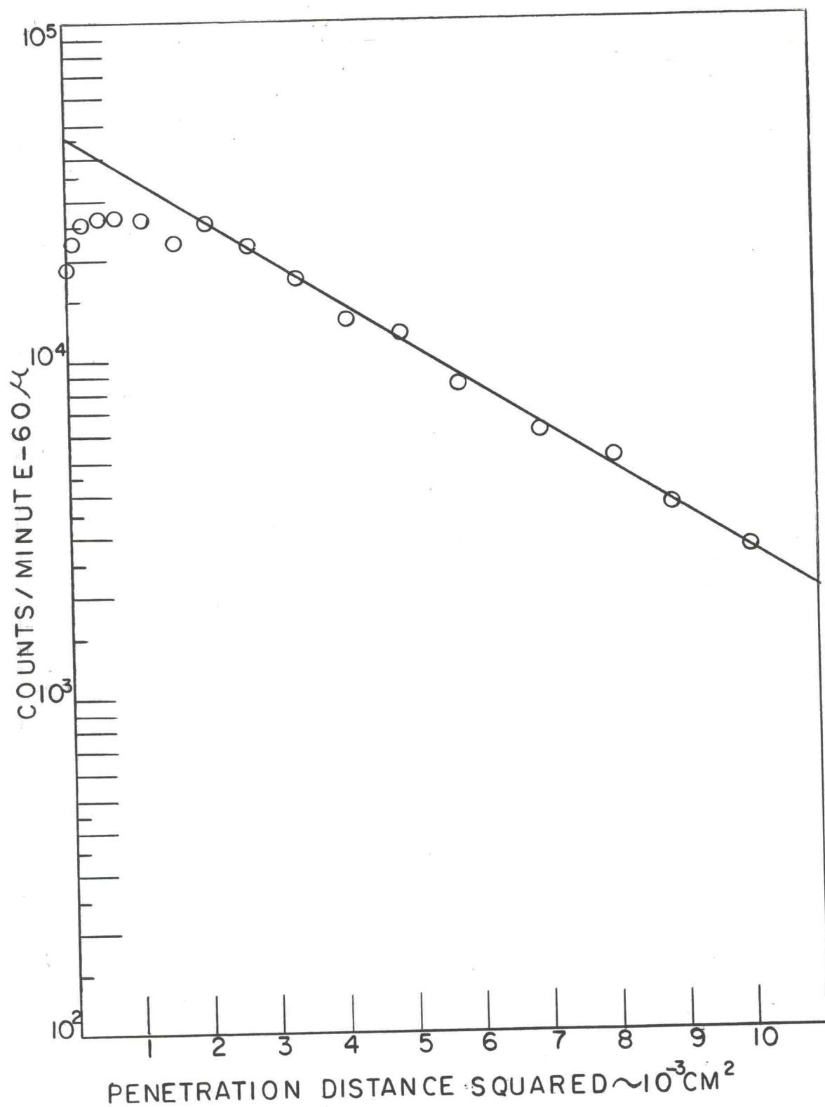
Figure 8. Solute Penetration Curve, Sample No. 88-- Annealed at 24 kb. pressure and 694^\circ\text{K} for 1.63 \times 10^4 sec
